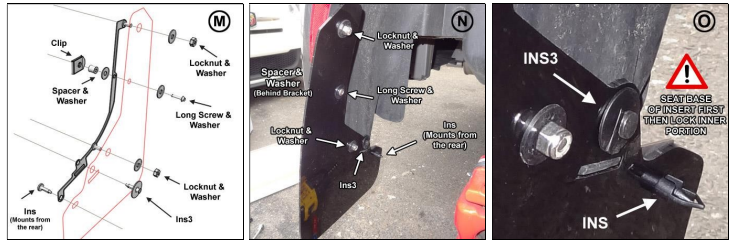
FRONT MOUNTING DIAGRAM
