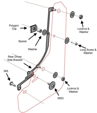
REAR MOUNTING DIAGRAM
