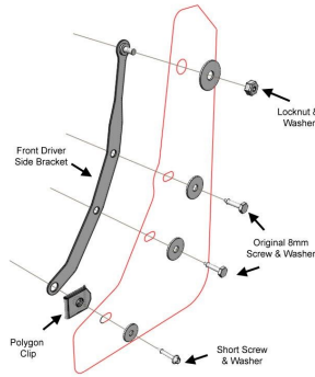
FRONT MOUNTING DIAGRAM
