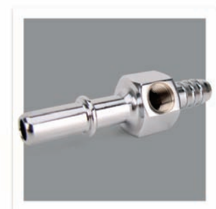
Supplied fuel line quick connectors make installation on the SRT8 easy with no cutting or drilling needed.
